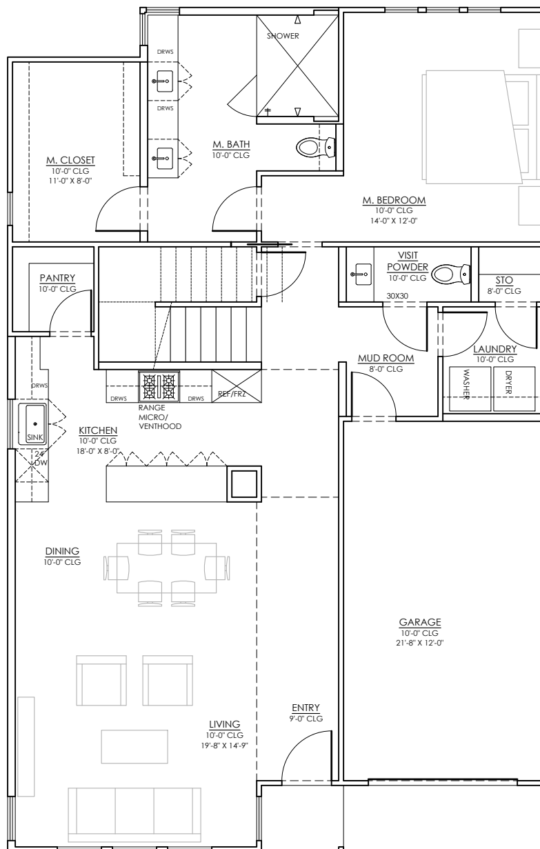
1 FIRST FLOOR PLAN UNIT A Scale: NTS
