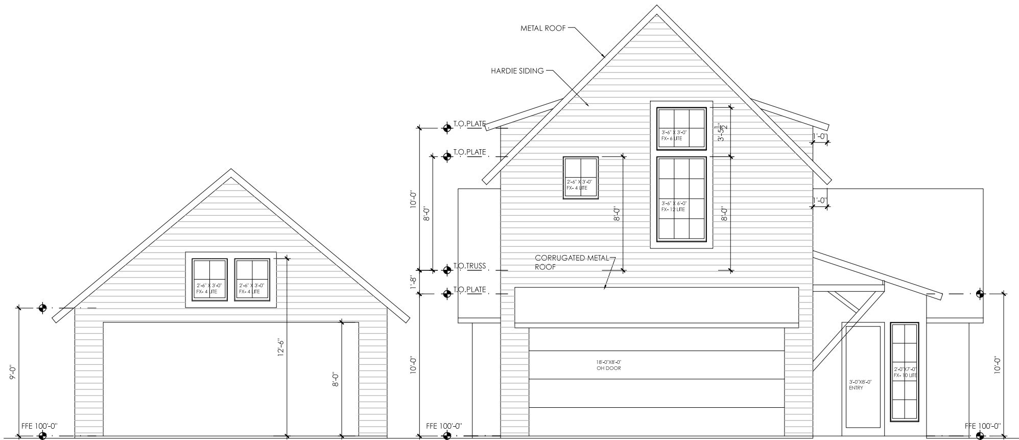
1 FRONT ELEVATION Scale: 3/32"=1'-0"
