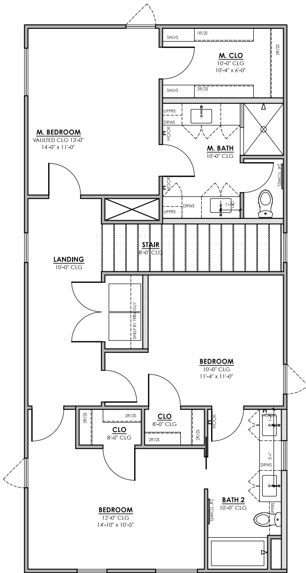
2 SECOND FLOOR PLAN PRIMARY Scale: 1/8"=1'-0"
