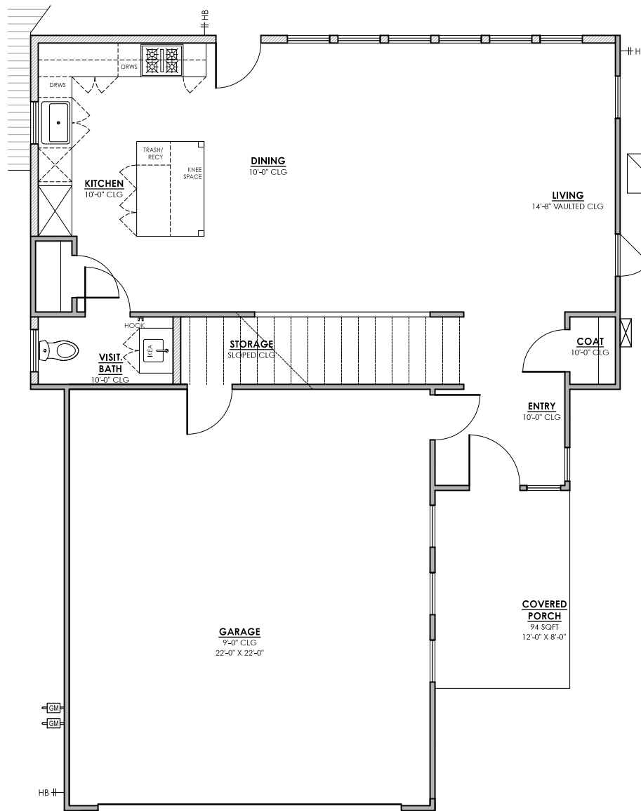
1 FIRST FLOOR PLAN PRIMARY Scale: 1/8"=1'-0"
