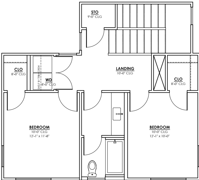
2 SECOND FLOOR PLAN Scale: 1/8"=1'-0"
