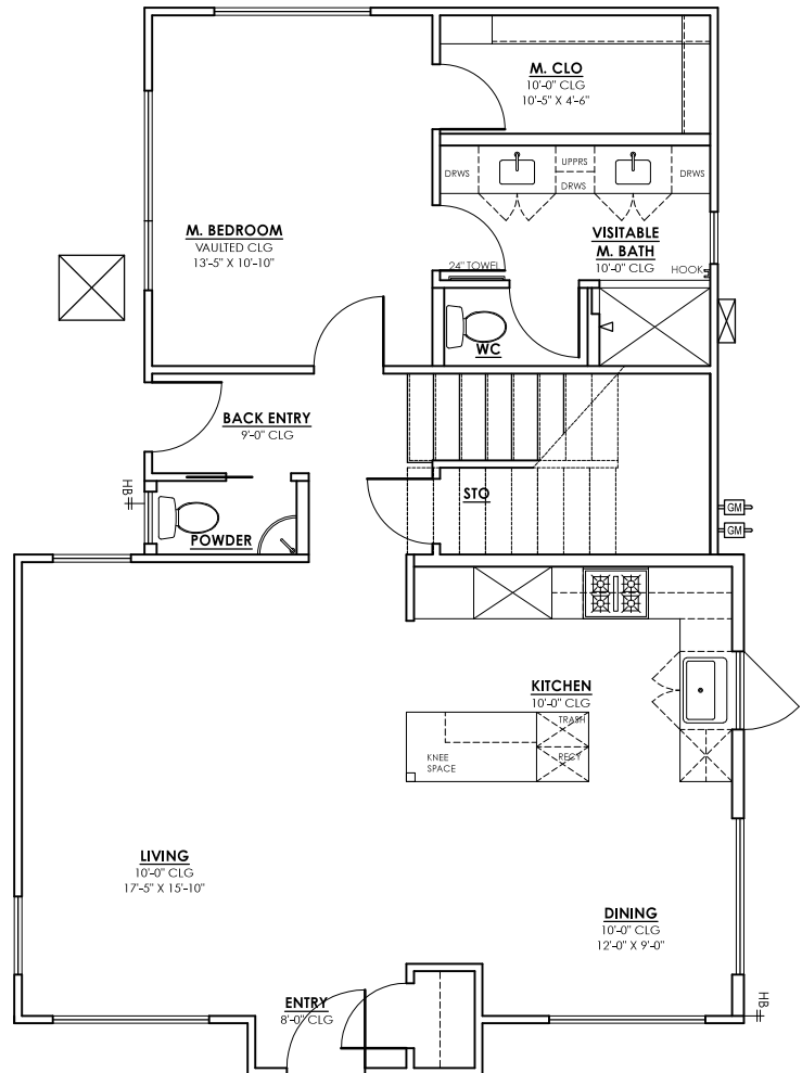
1 FIRST FLOOR PLAN Scale: 1/8"=1'-0"
